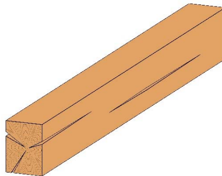
Figure 1 The width of seasoning checks reduces as the check approaches the pith. Multiple checks may meet at the pith but this is not considered a split.
